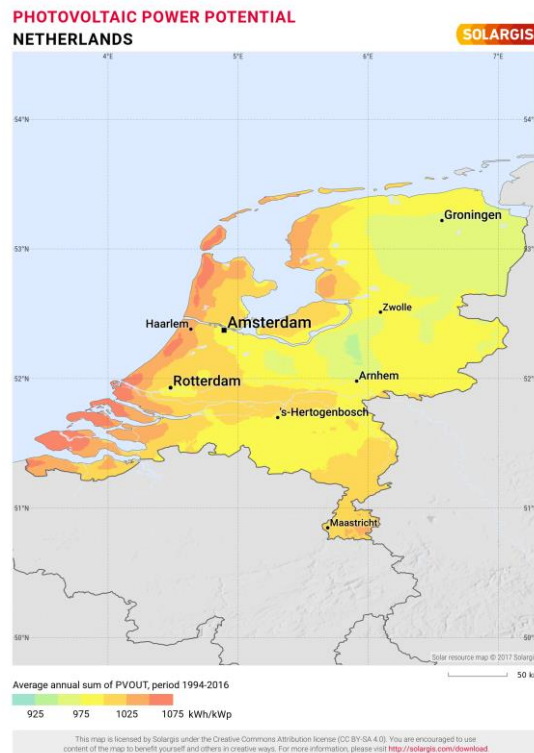
Figure 96 – Solar PV power potential for Netherlands (SOLARGIS, 2020).
