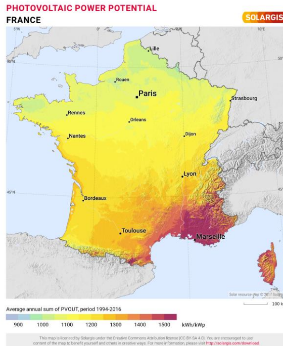
Figure 62 – Solar PV power potential in France (SOLARGIS, 2020).
