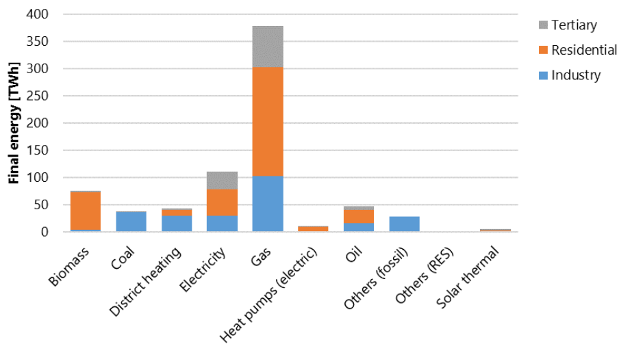
Figure 72 – Energy carrier split by sectoral demand in Italy [TWh] (Fleiter et al., 2017)
