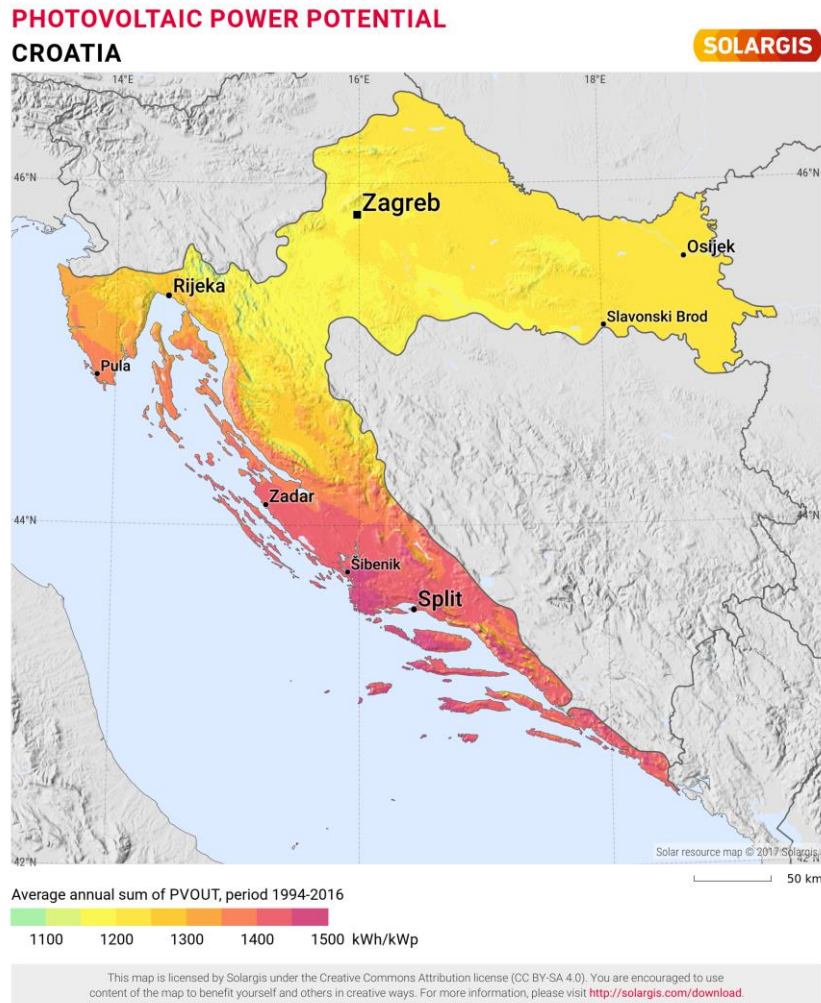
Figure 38 – The photovoltaic power potential in Croatia (SOLARGIS, 2020).
