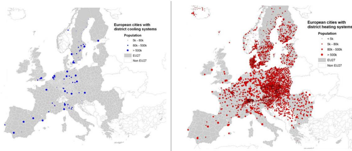
Figure 19 – District heating and cooling networks in Europe (Persson, 2013).
