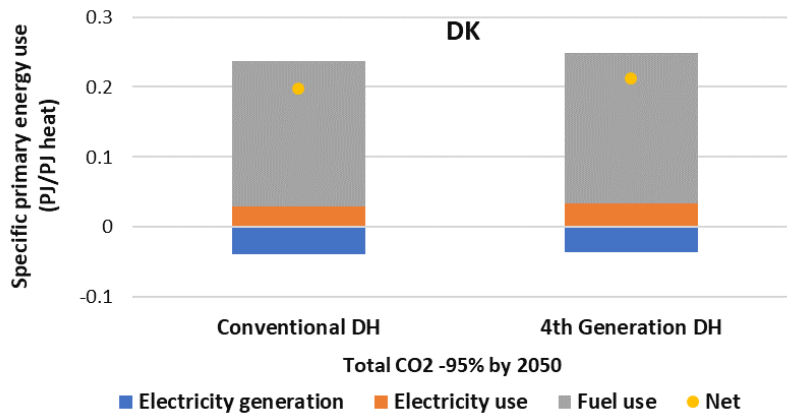
Figure 33 – The specific primary energy use, divided into fuel use, electricity generation and electricity use, of heat supply in the heating sector of Denmark in year 2050 in the FutureDH and ConventionalDH scenarios (with 95% CO 2 reduction by 2050).
