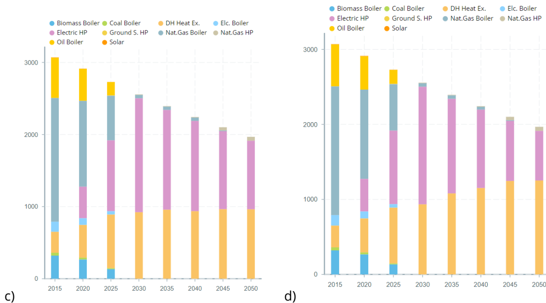
Figure 12 – End use heat demand in buildings (in PJ), covered by both individual heating solutions and DH, in Germany in the a) ConventionalDH technology development scenario (WEO-SD climate scenario), b) FutureDH technology development scenario (WEO-SD climate scenario), c) ConventionalDH technology development scenario (WEO-NP climate scenario), and d) FutureDH technology development scenario (WEO-NP climate scenario).
