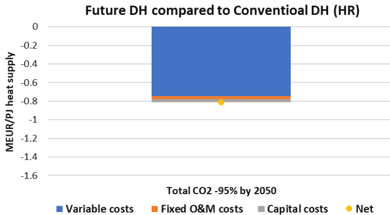
Figure 43 – The differences between the specific undiscounted Variable, Fixed O&M, and Capital (together with their total Net value) costs of heat supply in the heating sector of Croatia, averaged over the Years 2020-2050, in the FutureDH and ConventionalDH scenarios (with 95% CO 2 reduction by 2050).
