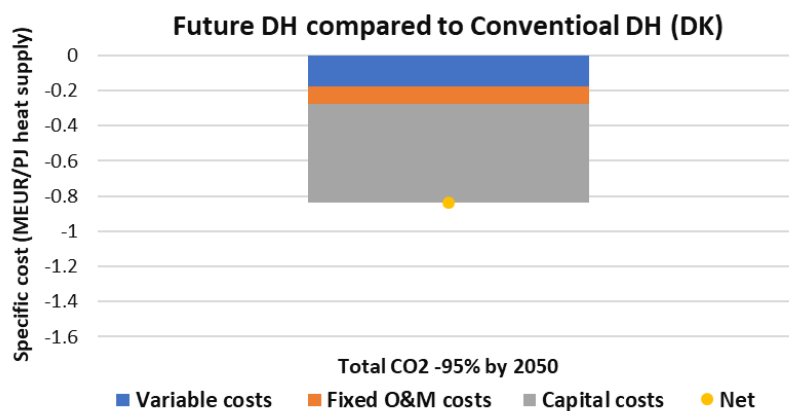
Figure 32 – The differences between the specific undiscounted Variable, Fixed O&M, and Capital (together with their total Net value) costs of heat supply in the heating sector of Denmark, averaged over the Years 2020-2050, in the FutureDH and ConventionalDH scenarios (with 95% CO2 reduction by 2050).
