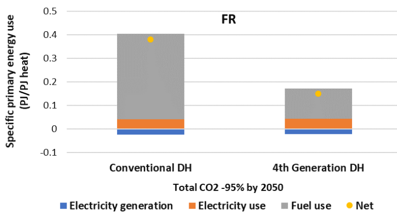
Figure 68 – The specific primary energy use, divided into fuel use, electricity generation and electricity use, of heat supply in the heating sector of France in year 2050 in the FutureDH and ConventionalDH scenarios (with 95% CO 2 reduction by 2050).
