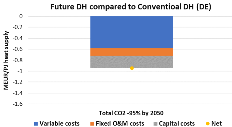
Figure 55 – The differences between the specific undiscounted Variable, Fixed O&M, and Capital (together with their total Net value) costs of heat supply in the heating sector of Germany, averaged over the Years 2020-2050, in the FutureDH and ConventionalDH scenarios (with 95% CO 2 reduction by 2050).
