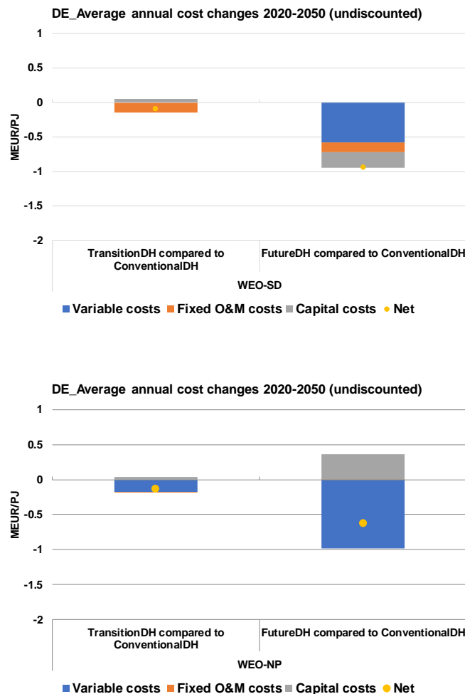
Figure 14 – Differences in the specific annual costs, divided into Variable, Fixed O&M and capital, averaged over the period 2020-2050, as a result of LTH sources use (in TransitionDH and FutureDH) and LTDH (In FutureDH) in the WEO-SD (top) and WEO-NP (bottom) scenarios in Germany.
