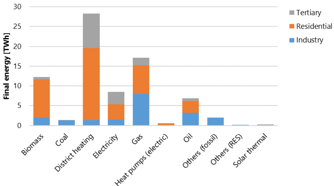
Figure 25 – Energy carrier split by sectoral demand in Denmark (Fleiter et al., 2017)
