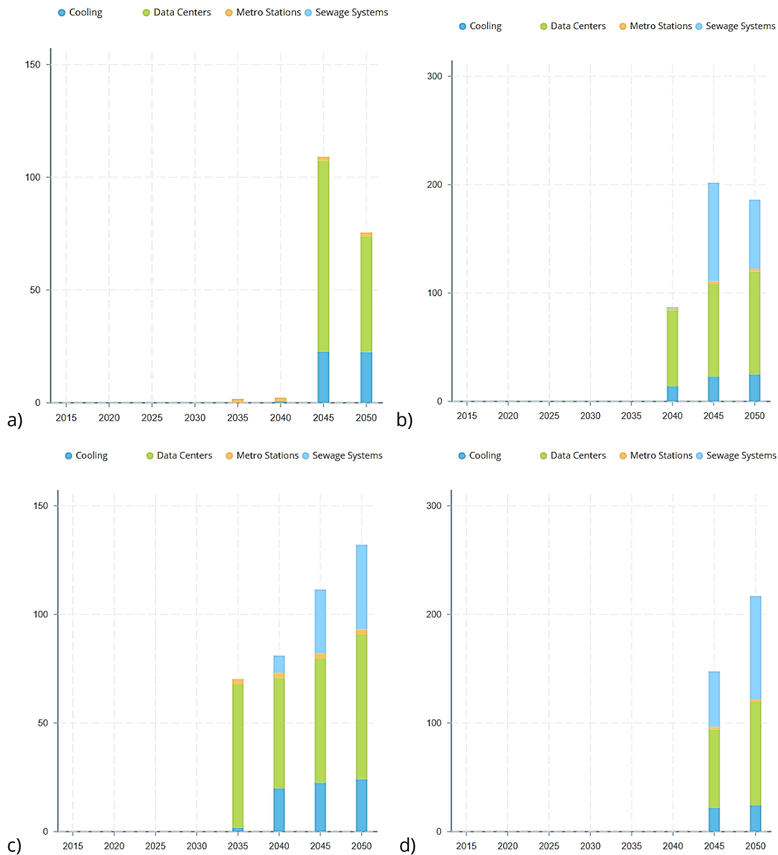
Figure 11 – The cost-efficient levels of utilization of the LTH sources (in Pj) in Germany in the a) TransitionDH technology development scenario (WEO-SD climate scenario), b) FutureDH technology development scenario (WEO-SD climate scenario), c) TransitionDH technology development scenario (WEO-NP climate scenario), and d) FutureDH technology development scenario (WEO-NP climate scenario).
