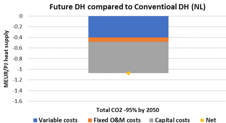
Figure 101 – The differences between the specific undiscounted Variable, Fixed O&M, and Capital (together with their total Net value) costs of heat supply in the heating sector of the Netherlands, averaged over the Years 2020-2050, in the FutureDH and ConventionalDH scenarios (with 95% CO 2 reduction by 2050).
