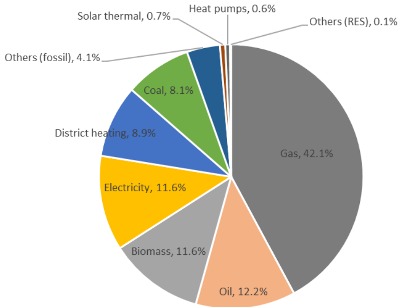
Figure 17 – Shares of energy carrier in the total final HC demand in EU28 (Fleiter et al., 2017).
