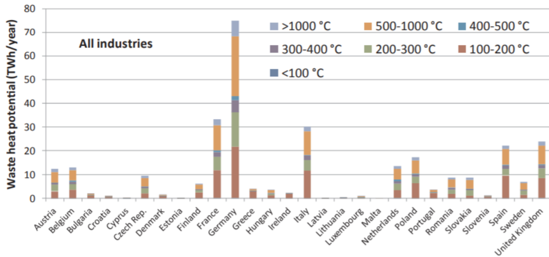
Figure 22 – Industrial waste heat potential in each EU country per temperature level in all industries (Papapetrou et al., 2018a).
