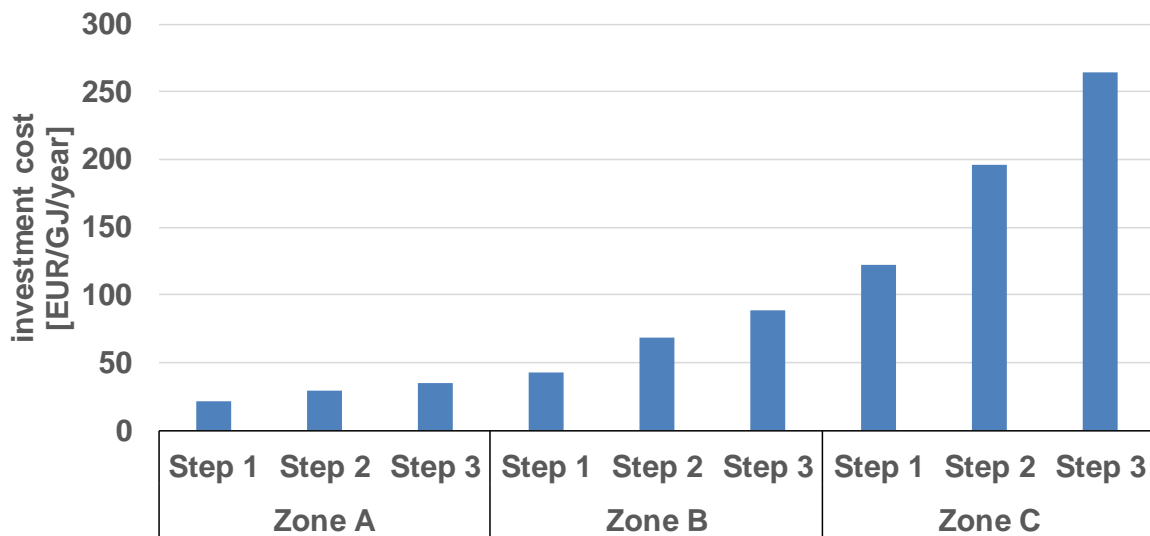
Figure 109 – DH network investment cost in different country zones. Each heat density zone has three cost levels (steps) which is linked to specific potentials.
