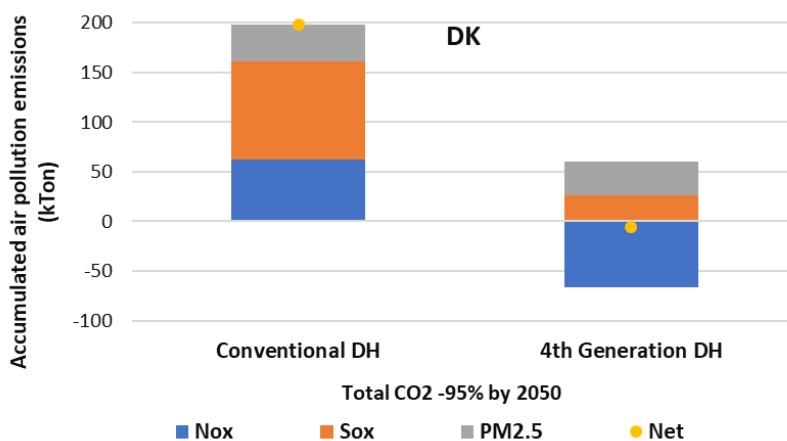
Figure 34 – The accumulated air pollutant emissions (NO x , SO x , PM 2.5 ) attributed to heat supply in the heating sector of Denmark over the period 2020-2050 in the FutureDH and ConventionalDH scenarios (with 95% CO 2 reduction by 2050).
