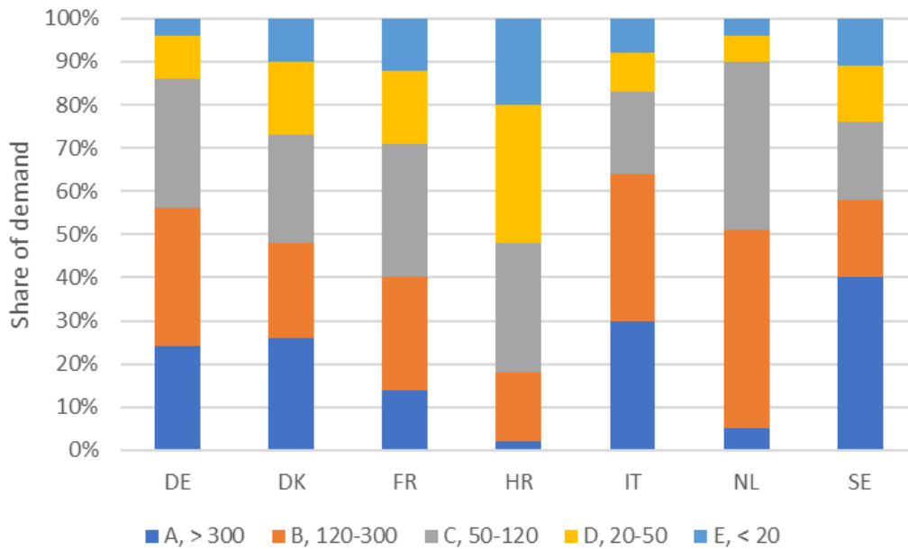
Figure 108 – Share of heat demand for different heat density levels (PJ/km 2 ) and corresponding model zones A-E.
