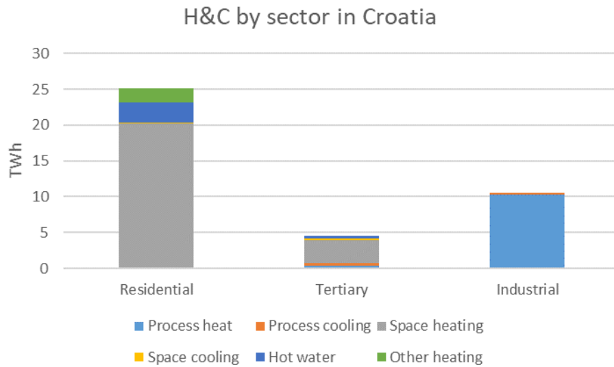
Figure 35 – HC by sector and country (Fleiter et al., 2017).
