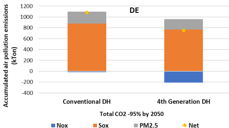
Figure 57 – The accumulated air pollutant emissions (NO x , SO x , PM 2.5 ) attributed to heat supply in the heating sector of Germany over the period 2020-2050 in the FutureDH and ConventionalDH scenarios (with 95% CO 2 reduction by 2050).
