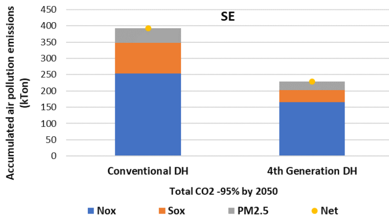
Figure 91 – The accumulated air pollutant emissions (NO x , SO x , PM 2.5 ) attributed to heat supply in the heating sector of Sweden over the period 2020-2050 in the FutureDH and ConventionalDH scenarios (with 95% CO 2 reduction by 2050).
