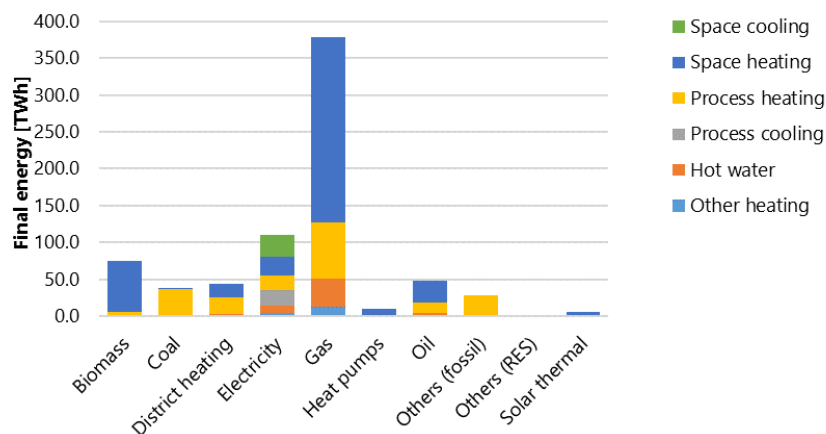
Figure 71 – Energy carrier for the final HC demand for all sectors in Italy [TWh] (Fleiter et al., 2017)
