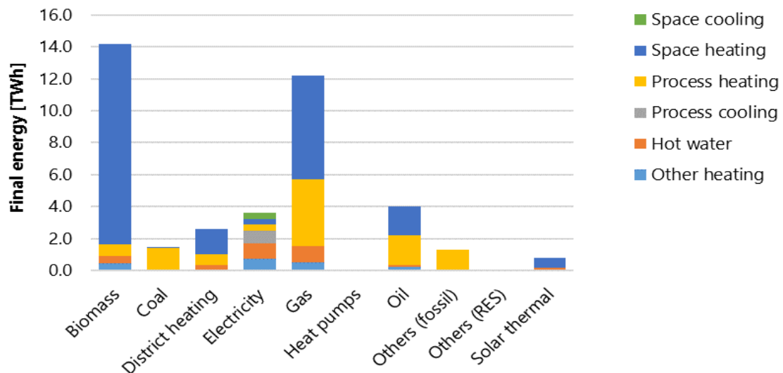
Figure 36 – Energy carrier for the final HC demand for all sectors in Croatia [TWh] (Fleiter et al., 2017).
