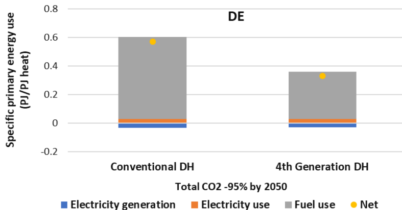
Figure 56 – The specific primary energy use, divided into fuel use, electricity generation and electricity use, of heat supply in the heating sector of Germany in year 2050 in the FutureDH and ConventionalDH scenarios (with 95% CO 2 reduction by 2050).
