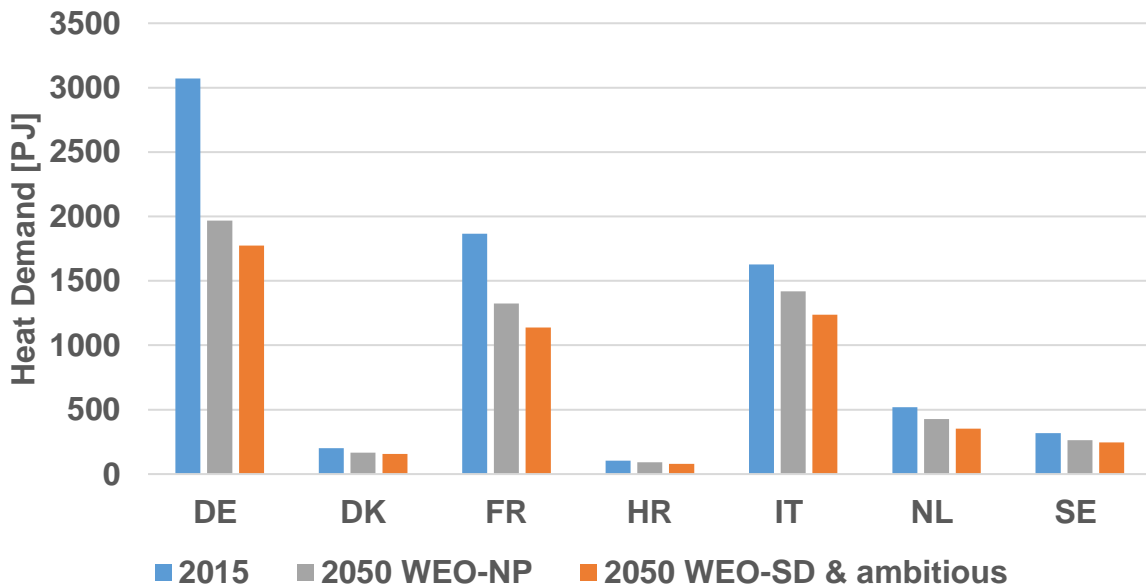
Figure 105 – Total demand in model base year (2015) and in 2050 for three climate policy scenarios.
