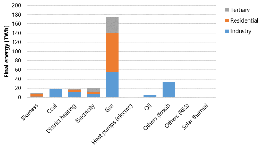
Figure 94 – Energy carrier split by sectoral demand in Netherlands [TWh] (Fleiter et al., 2017).
