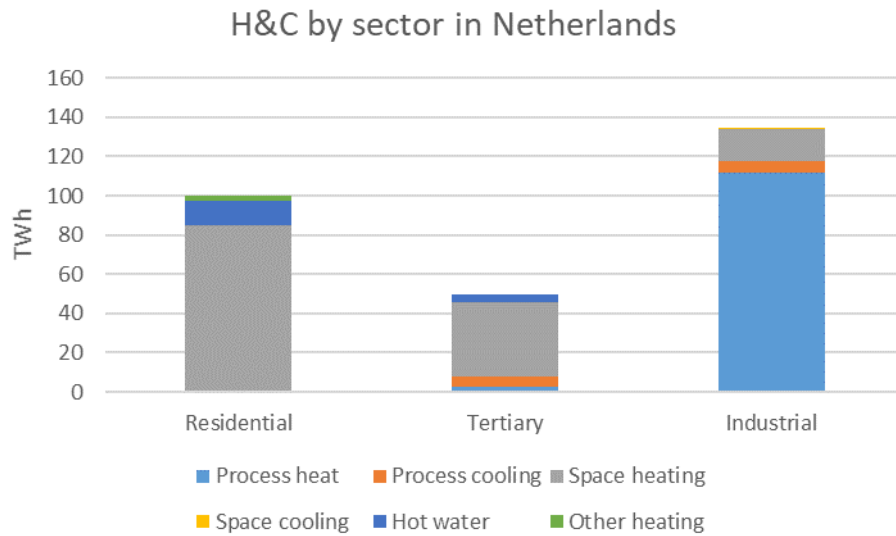
Figure 92 – HC by sector in Netherlands (Fleiter et al., 2017).
