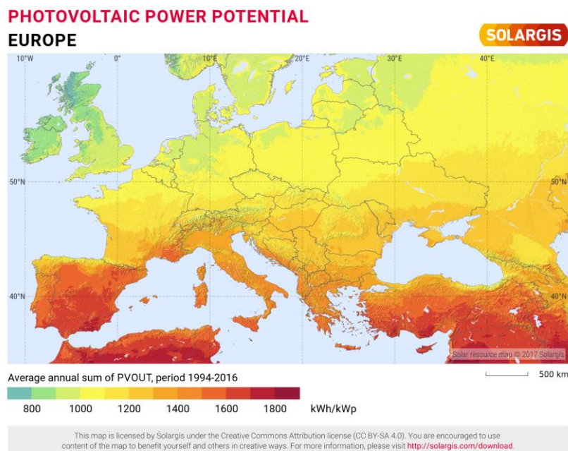
Figure 20 – Photovoltaic power potential in Europe (SOLARGIS, 2020).
