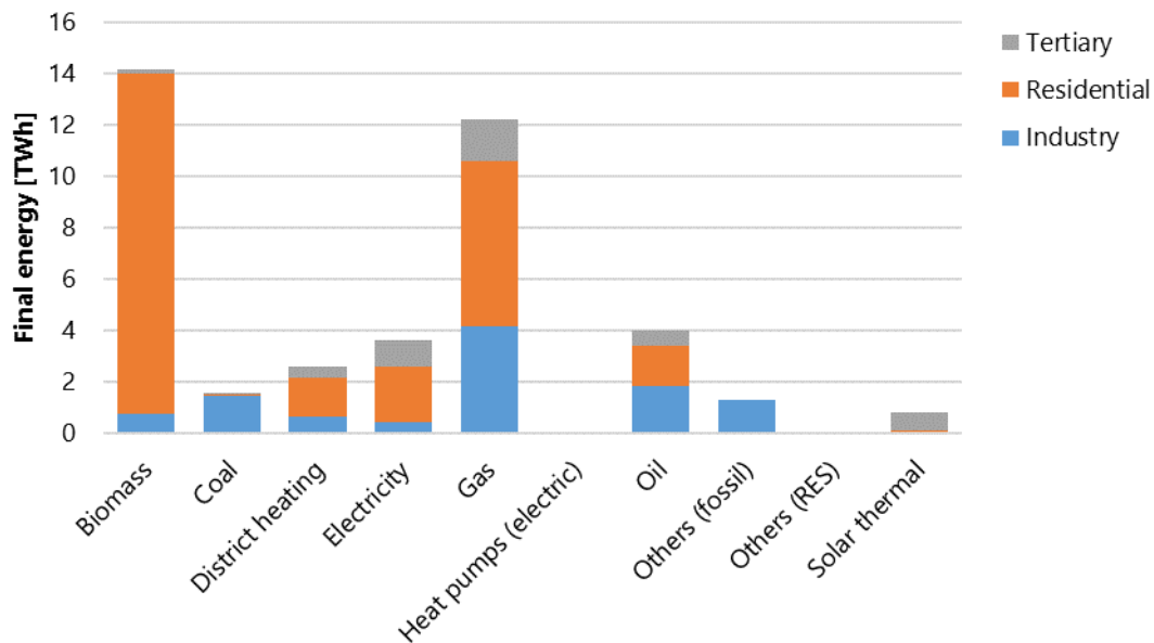
Figure 37 – Energy carrier split by sectoral demand in Croatia [TWh] (Fleiter et al., 2017).
