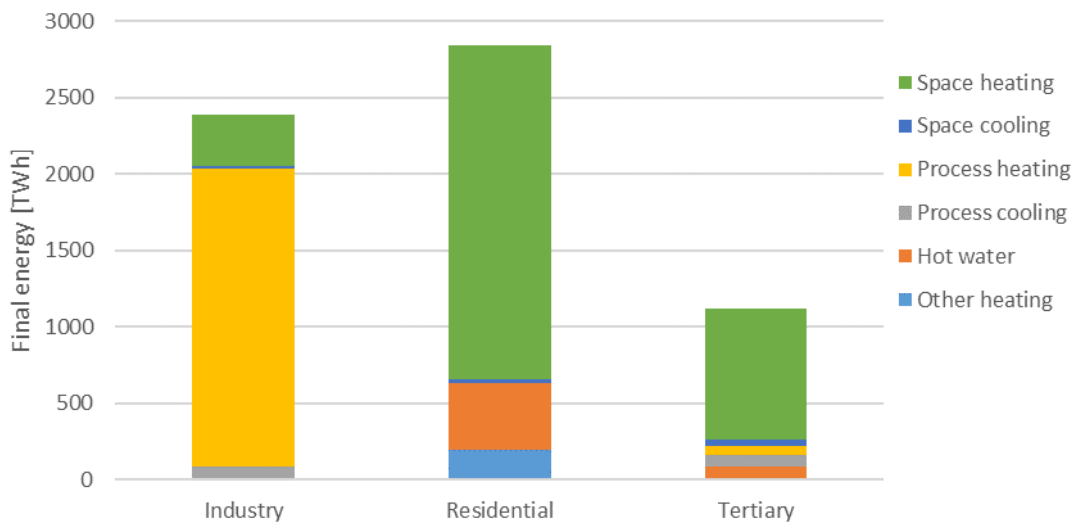
Figure 18 – Shares of type of heat in final HC by sector [TWh] (Fleiter et al., 2017).
