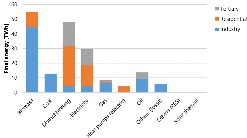
Figure 83 – Energy carrier split by sectoral demand in Sweden [TWh] (Fleiter et al., 2017).
